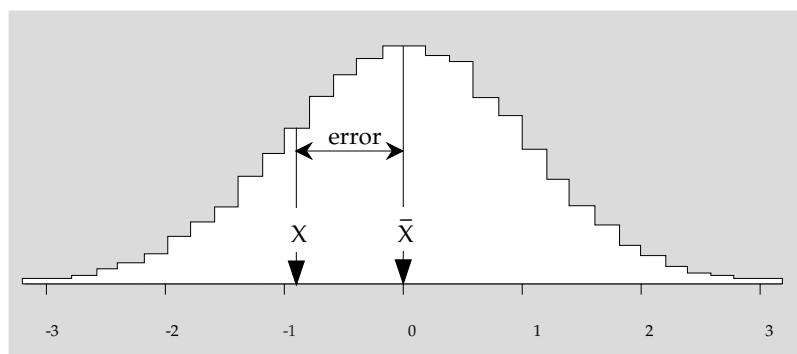
Figure 6: The Error of a Single Measurement
