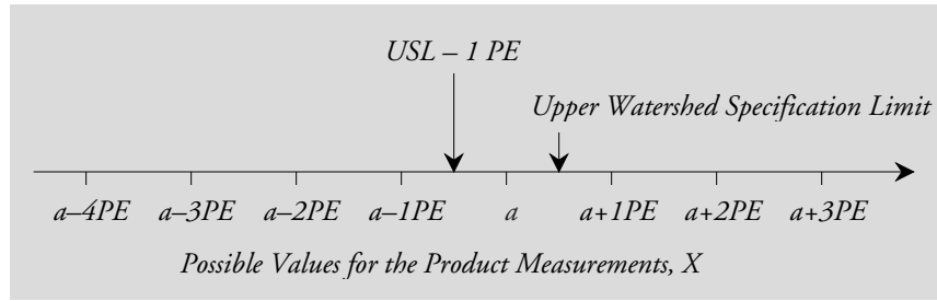
Figure 15: Watershed Specification Tightened by One Probable Error
